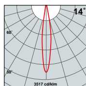
70W MH
