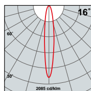
150W MH
