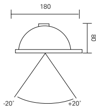
dimension (mm)
