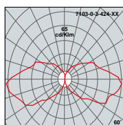
PLC 1x26W
