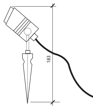
6W LED
